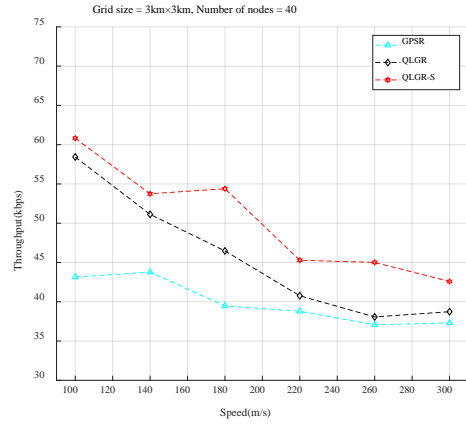
(c) (d) Fig. 9. Relationship between node speed and throughput
