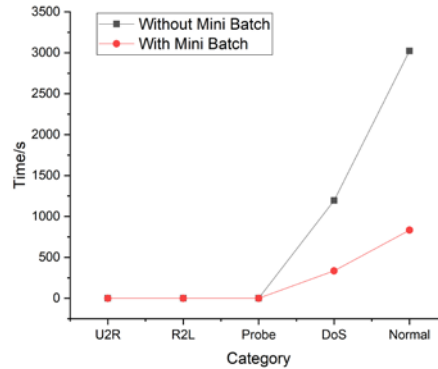
Fig. 5. Time analysis of improved the KNN outlier detection algorithm on KDD Cup 1999 dataset
