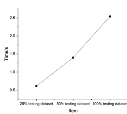
Fig. 13. Detection efficiency of the proposed algorithm
