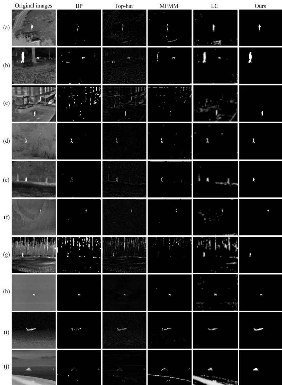
Fig. 8. Qualitative comparison results between the proposed method and other state-of-the-art approaches.
