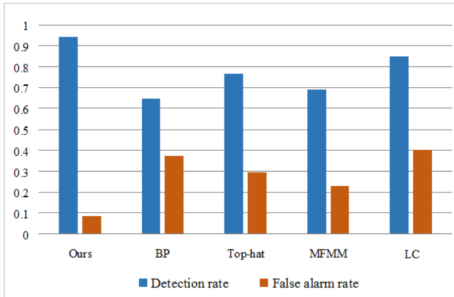
Fig. 9. Quantitative comparison results between the proposed method and other state-of-the-art approaches.
