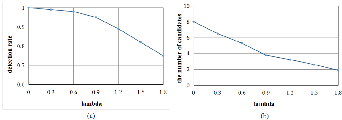
Fig. 5. Analysis of the parameter \lambda . (a) Effect of \lambda on detection rate. (b) Effect of \lambda on the number of candidate target regions.
