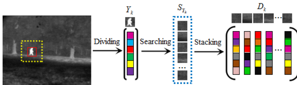
Fig. 2. Dissimilar dictionary learning process.
