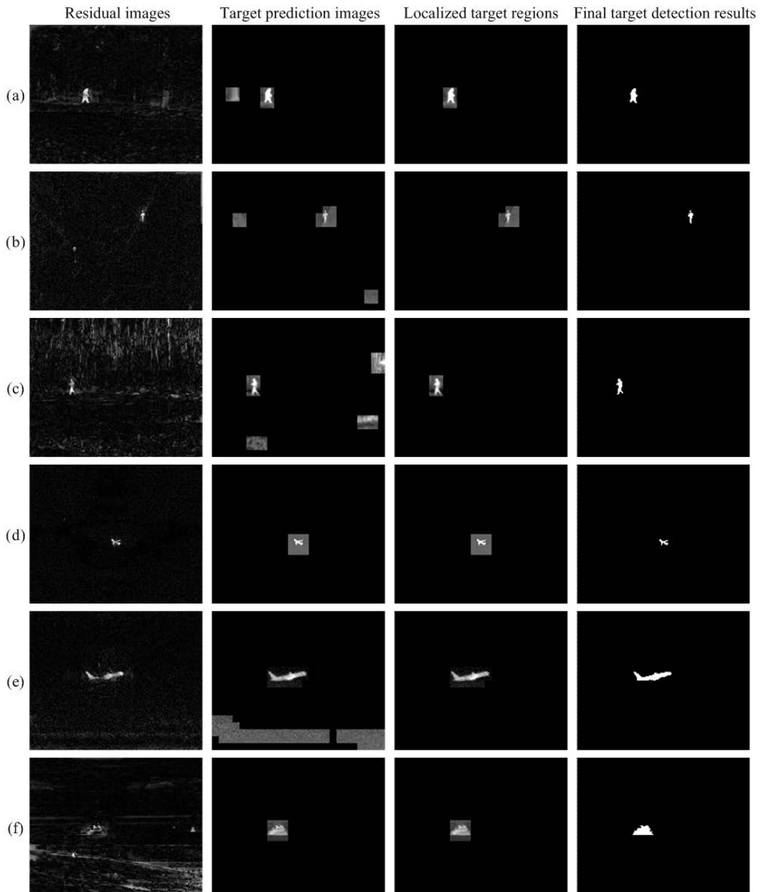
Fig. 7. Target detection results of the proposed method.
