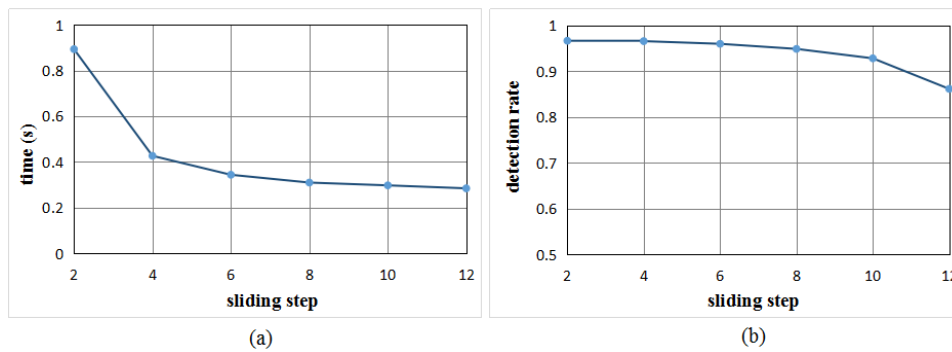
Fig. 4. Analysis of the parameter step . (a) Effect of step on detection efficiency. (b) Effect of step on detection rate.
