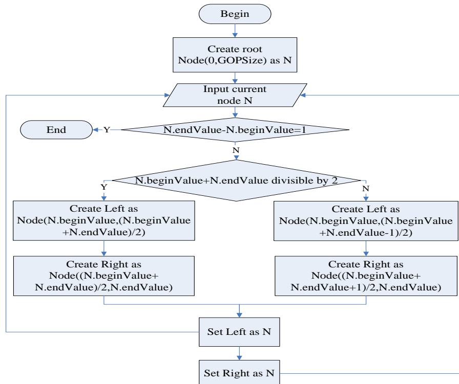
Fig. 5. Creation flow chart for the binary tree
