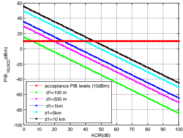
Fig. 9. PIB_{WLGCC} as a function of ACIR value for five separation distances between WLGCC-TX and DB-SS ( d_2 )
