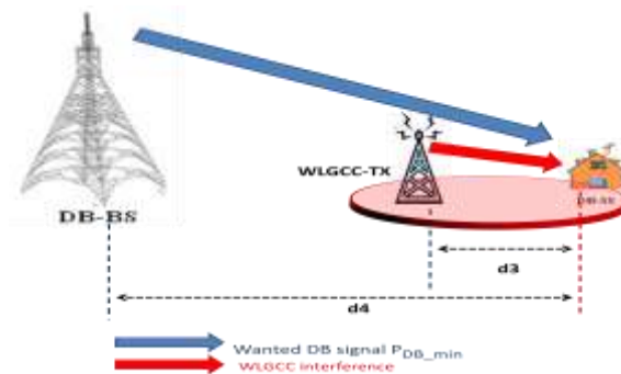
Fig. 7. Compatibility between the WLGCC-TX and DB-SS
