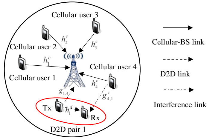
Fig. 1. System model of underlaying D2D communication.
