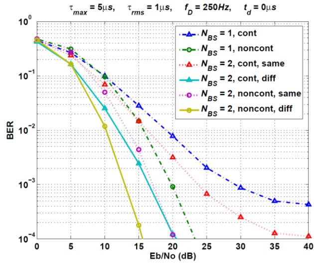
Fig. 3. BER comparison of different soft hand-over strategies when a mobile is located at r (3km) which corresponds to 0 \mu s .
