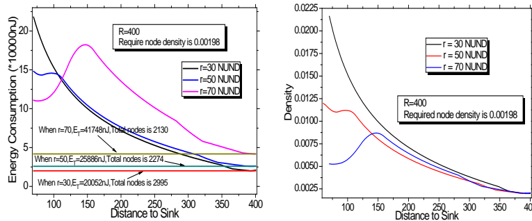
Fig. 4. Required sensor nodes under different cluster radii to achieve balanced energy consumption Fig. 5. Node densities in different areas under different cluster radii to achieve balanced energy
