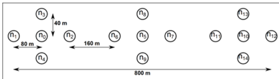
Fig. 9. Network topology
