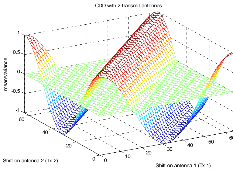
Fig. 5. Mean and variance of the transmitted signal with two transmit antennas.
